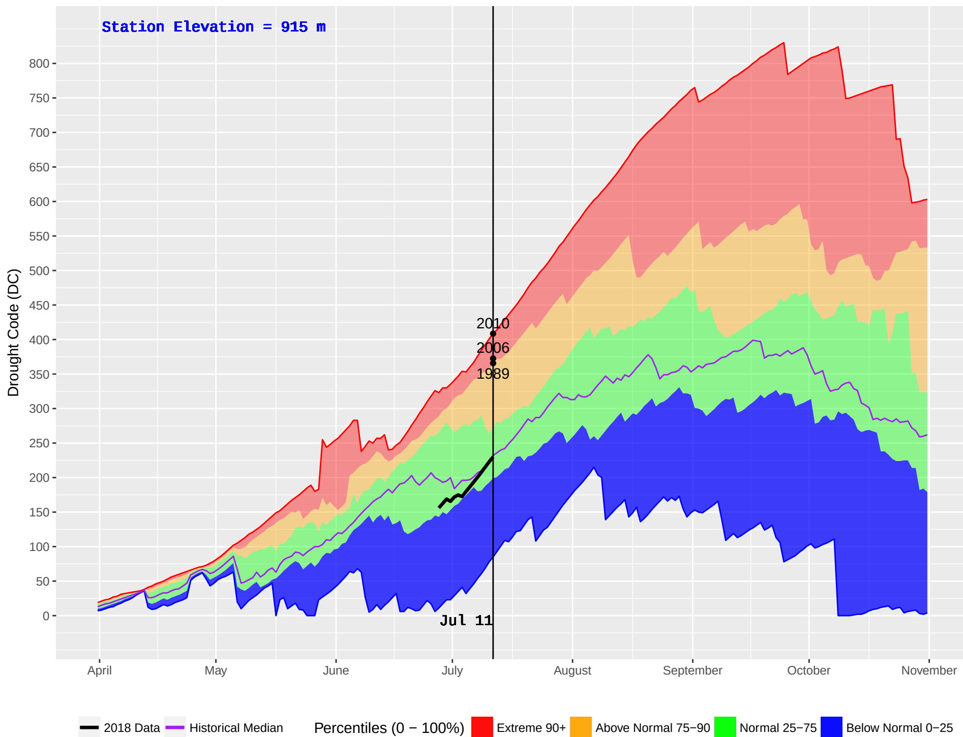
LEO CREEK (171) : Historical (1989–2016) and Current (2018) Noon Drought Code (DC)
