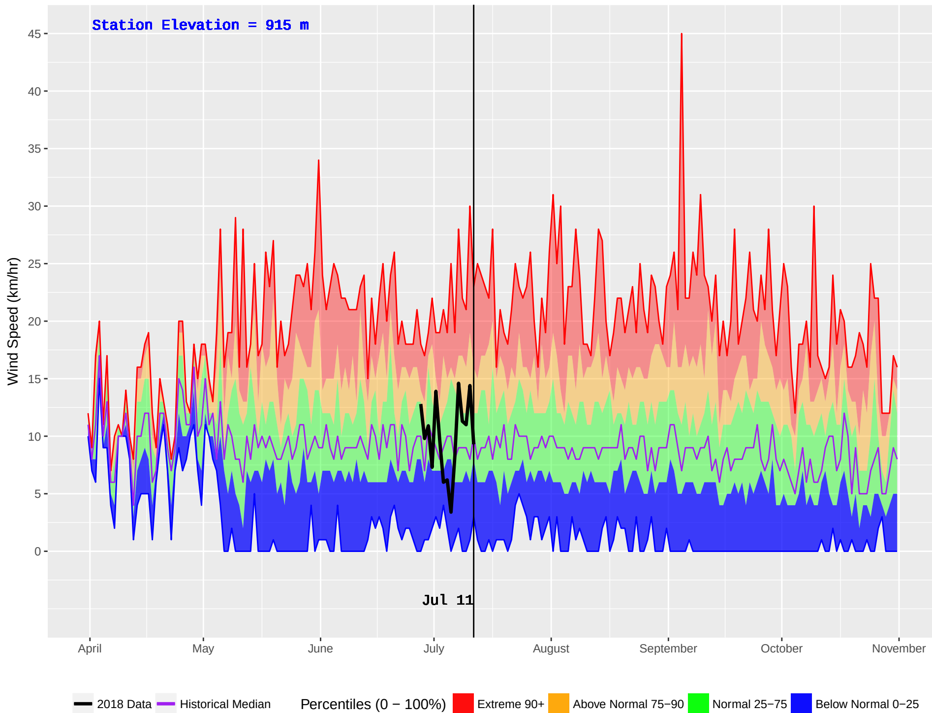
LEO CREEK (171) : Historical (1989–2016) and Current (2018) Noon Wind Speed
