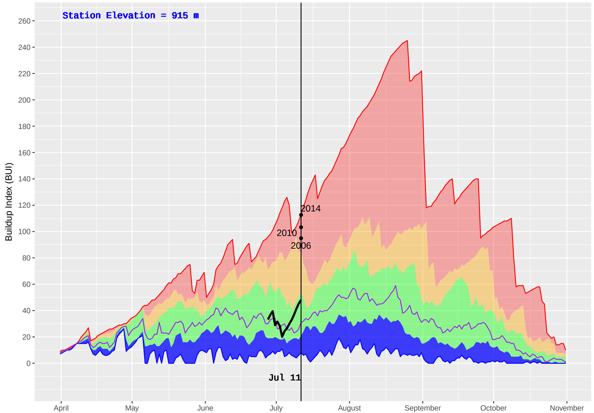
LEO CREEK (171) : Historical (1989–2016) and Current (2018) Noon Buildup Index (BUI)
